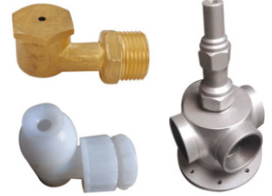
Brass/Eng. Plastic/ S.S. Nozzle and Sprinkler
