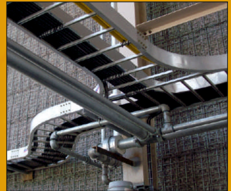
Cable Tray Installation
